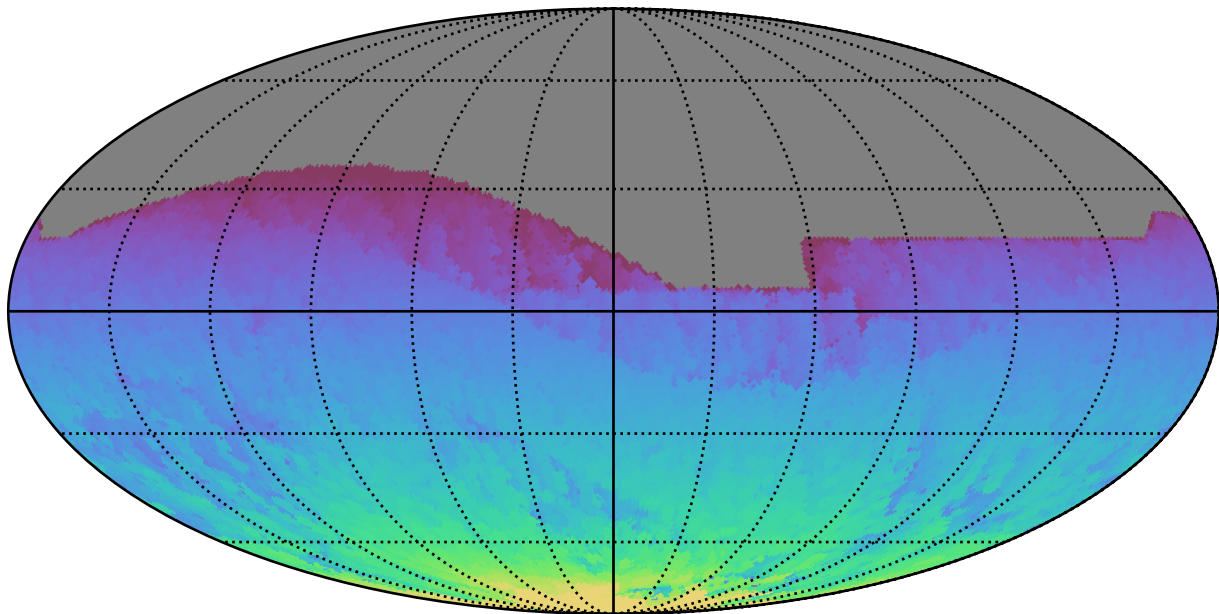
weather_cloudso4v3.4_10yrs All sky all bands: Max HA
