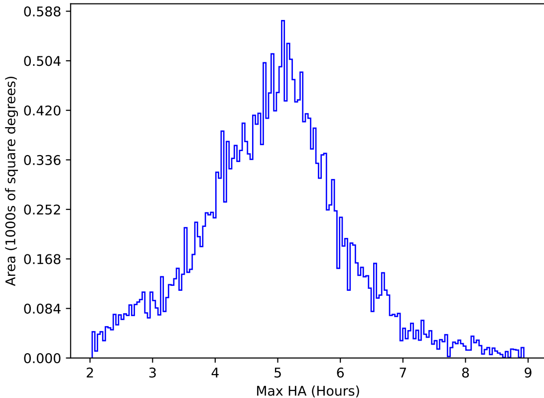
weather_cloudso4v3.4_10yrs All sky all bands: Max HA
