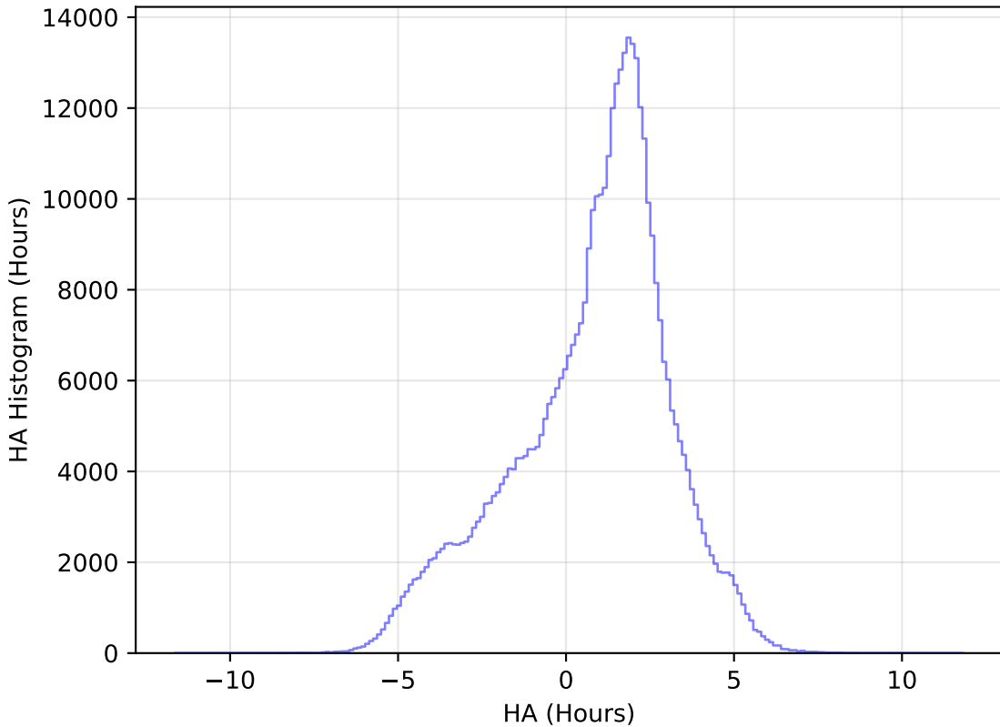
weather_cloudso4v3.4_10yrs WFD z band: HA Histogram
