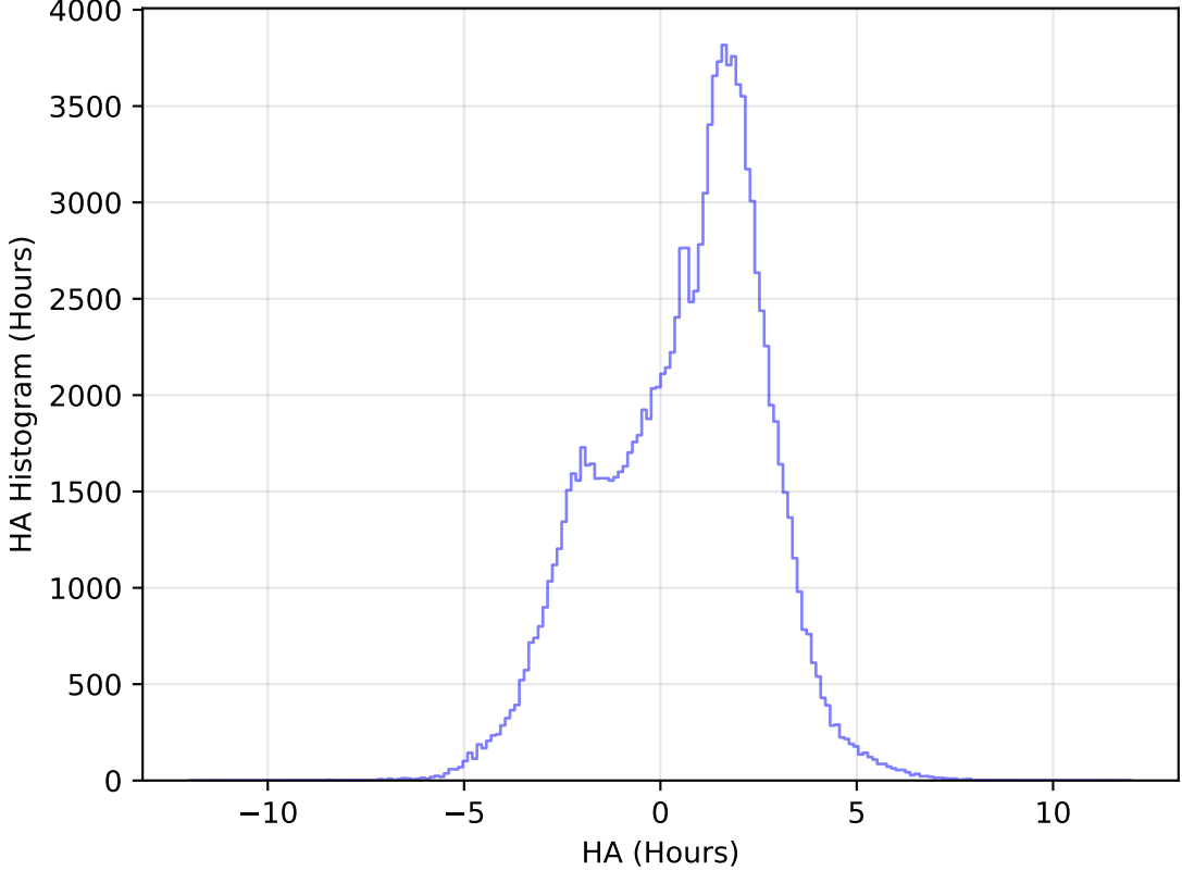
weather_cloudso4v3.4_10yrs WFD u band: HA Histogram
