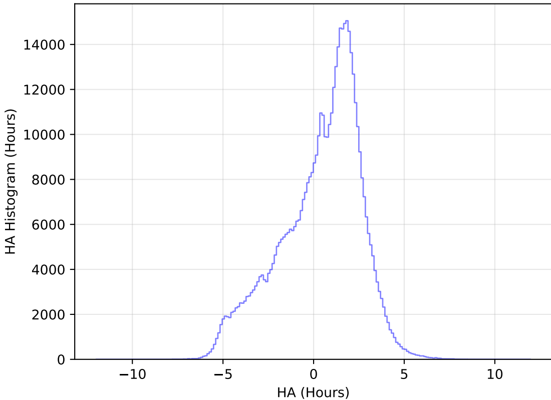
weather_cloudso4v3.4_10yrs WFD r band: HA Histogram
