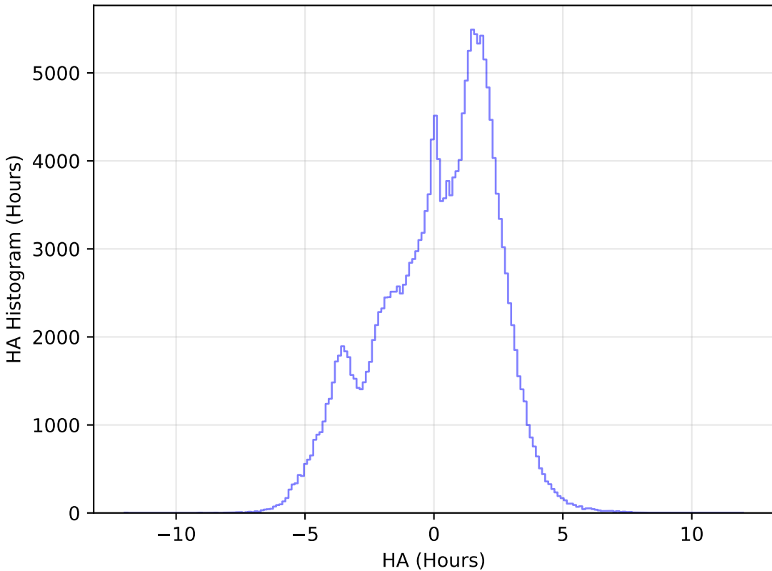
weather_cloudso4v3.4_10yrs WFD g band: HA Histogram
