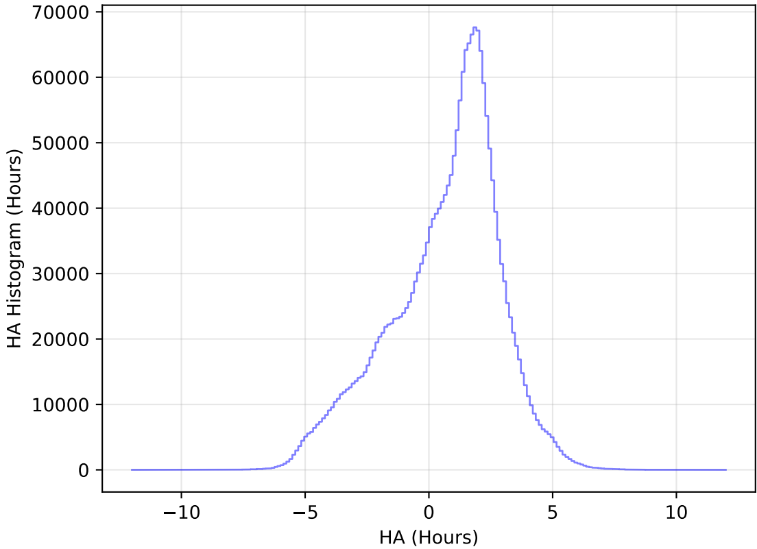
weather_cloudso4v3.4_10yrs WFD all bands: HA Histogram
