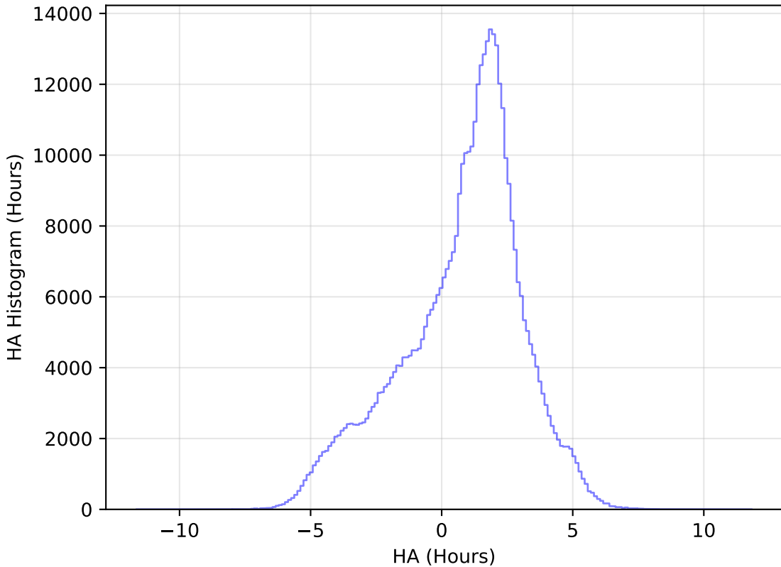
weather_cloudso4v3.4_10yrs All sky z band: HA Histogram
