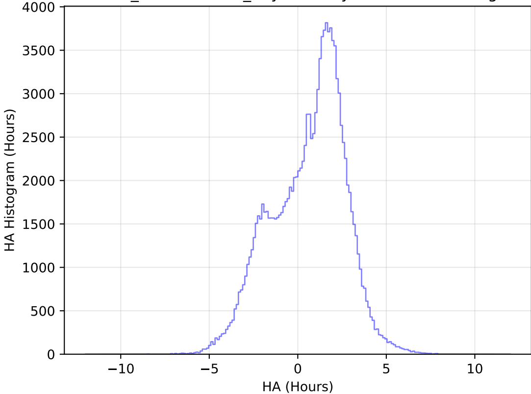
weather_cloudso4v3.4_10yrs All sky u band: HA Histogram
