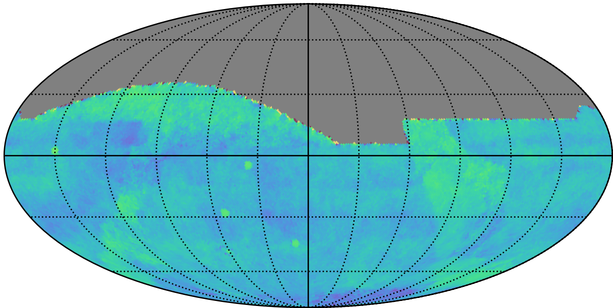
weather_cloudso4v3.4_10yrs gri All sky: Fraction of visits in pairs (20-90 min)
