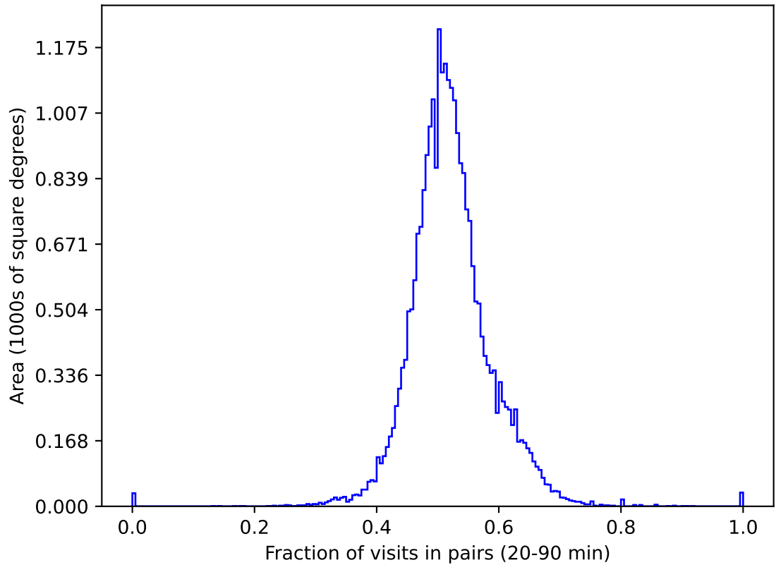
weather_cloudso4v3.4_10yrs gri All sky: Fraction of visits in pairs (20-90 min)
