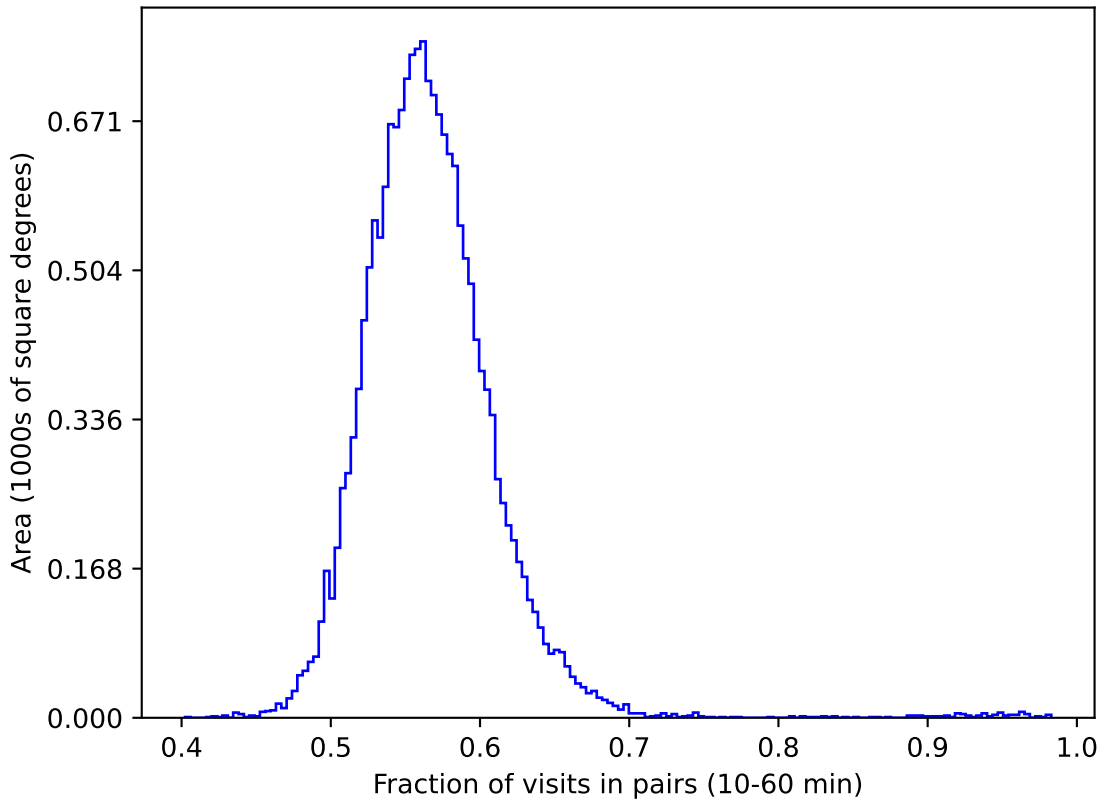
weather_cloudso4v3.4_10yrs gri WFD: Fraction of visits in pairs (10-60 min)
