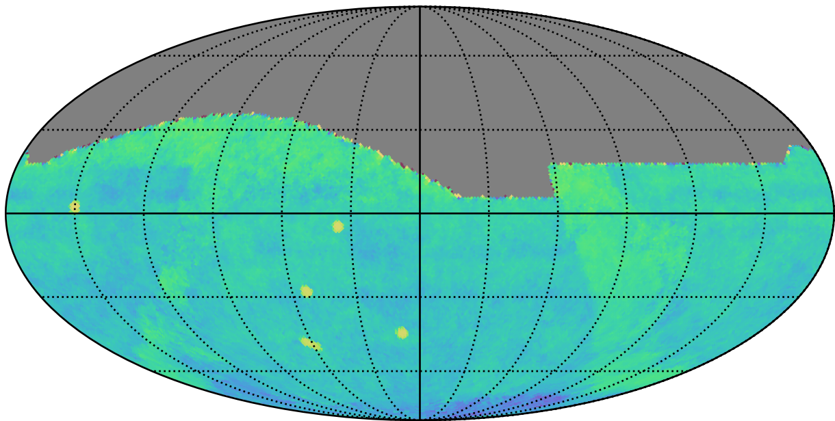
weather_cloudso4v3.4_10yrs gri All sky: Fraction of visits in pairs (10-60 min)
