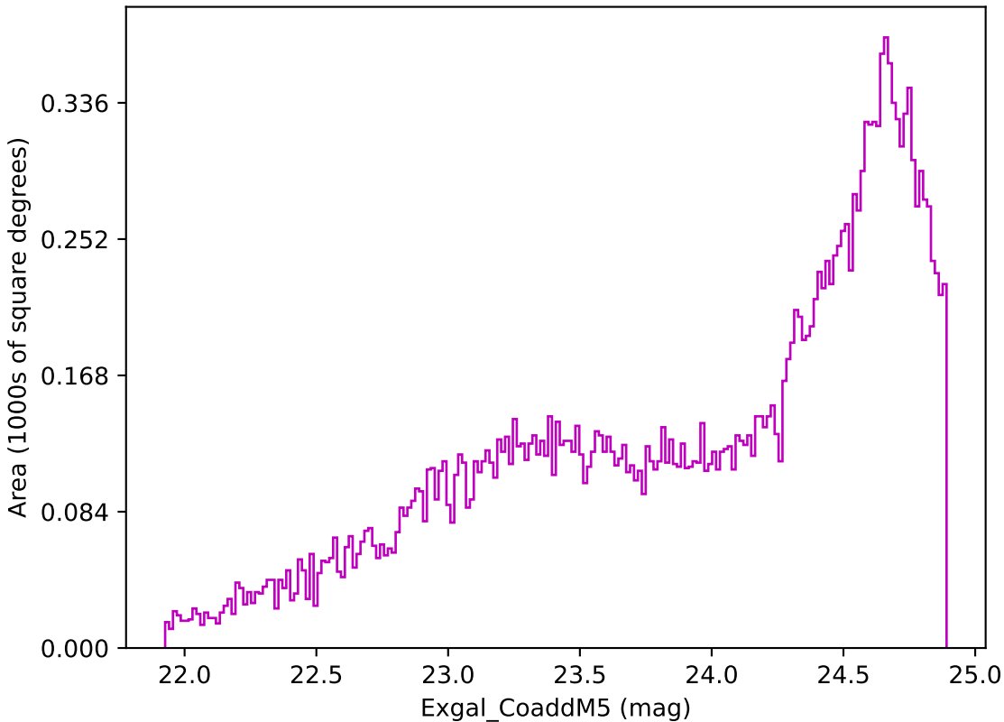
weather_cloudso4v3.4_10yrs Yr 3-4 z band: Exgal_CoaddM5
