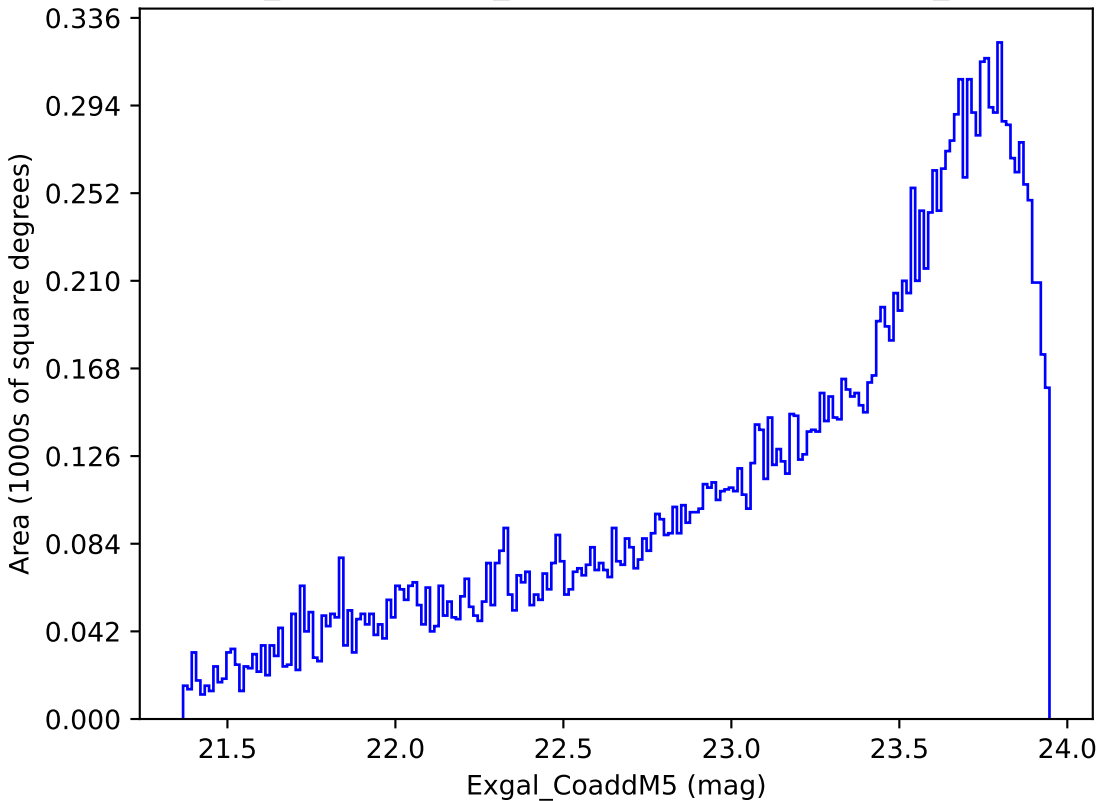
weather_cloudso4v3.4_10yrs Yr 3-4 y band: Exgal_CoaddM5
