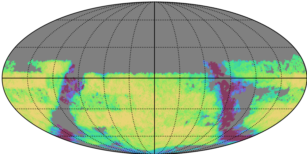
weather_cloudso4v3.4_10yrs Yr 3-4 u band: Exgal_CoaddM5
