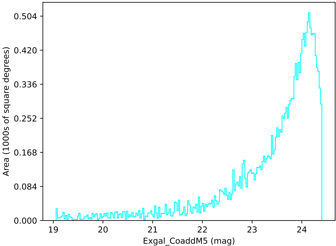
weather_cloudso4v3.4_10yrs Yr 3-4 u band: Exgal_CoaddM5
