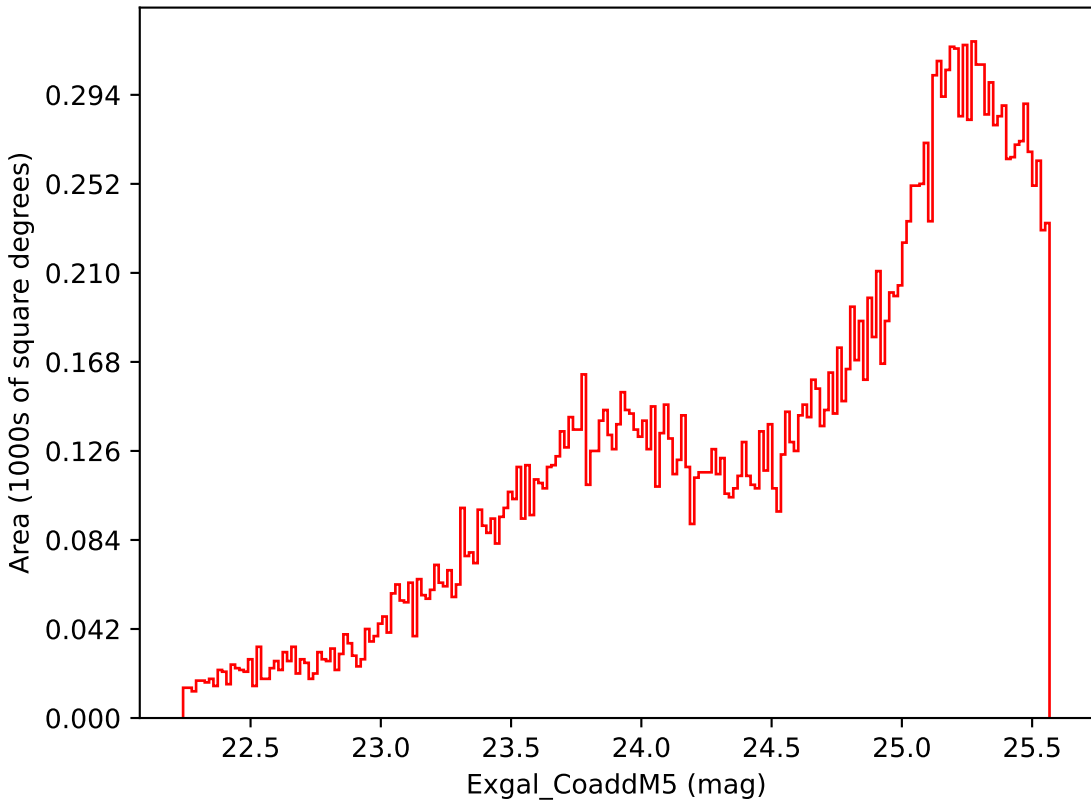
weather_cloudso4v3.4_10yrs Yr 3-4 i band: Exgal_CoaddM5
