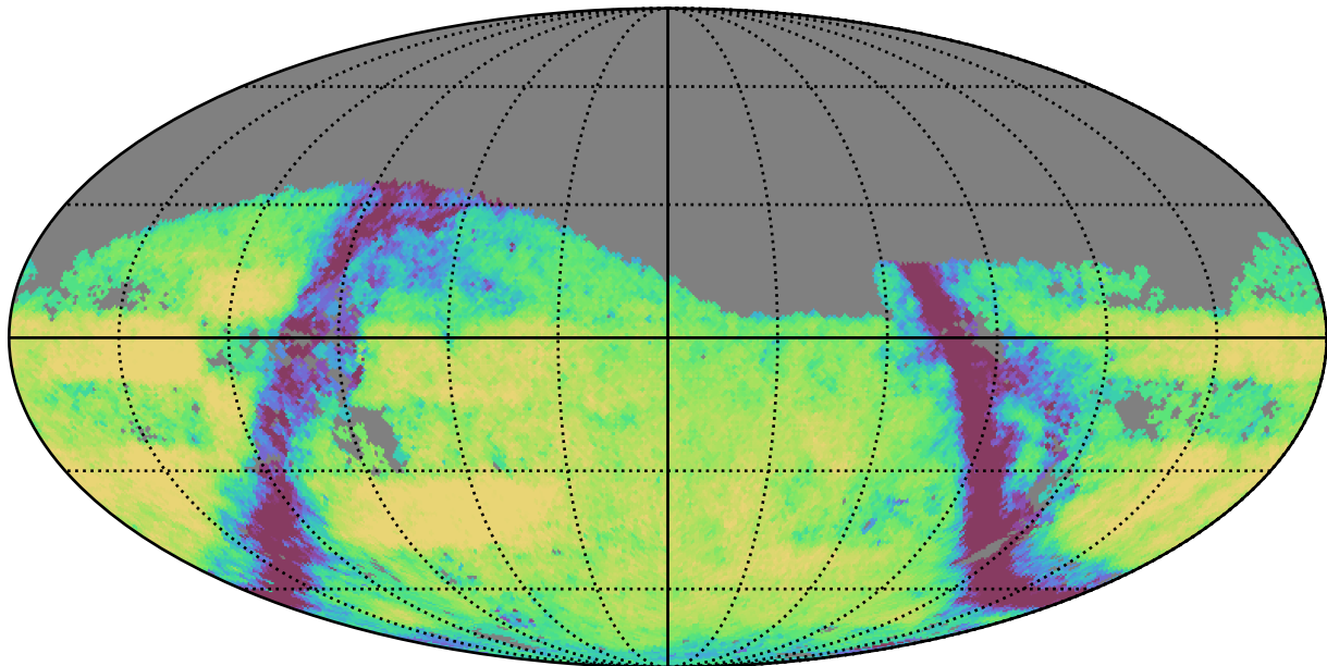
weather_cloudso4v3.4_10yrs Yr 3-4 g band: Exgal_CoaddM5
