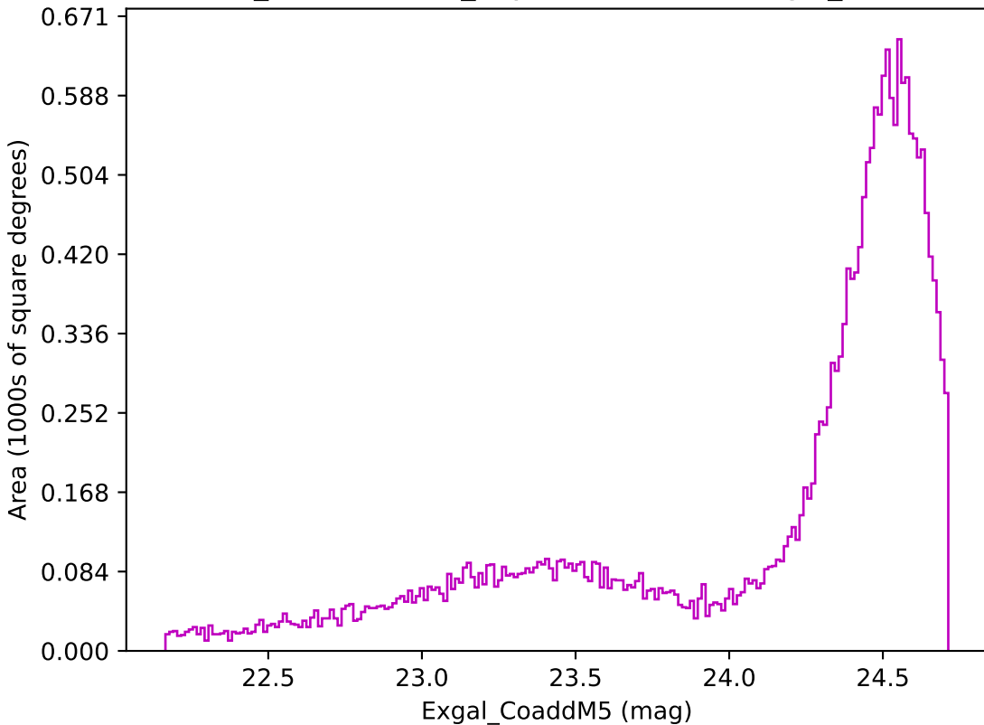
weather_cloudso4v3.4_10yrs Yr 1 z band: Exgal_CoaddM5
