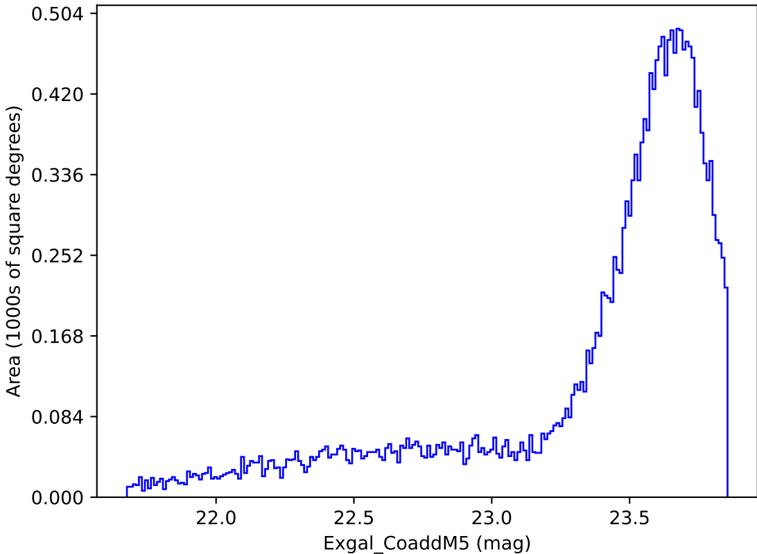
weather_cloudso4v3.4_10yrs Yr 1 y band: Exgal_CoaddM5
