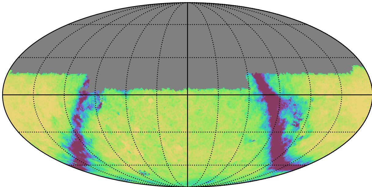
weather_cloudso4v3.4_10yrs Yr 1 u band: Exgal_CoaddM5
