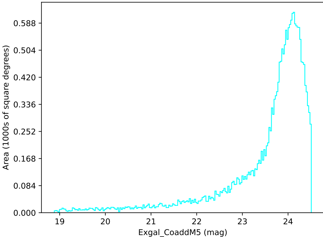
weather_cloudso4v3.4_10yrs Yr 1 u band: Exgal_CoaddM5
