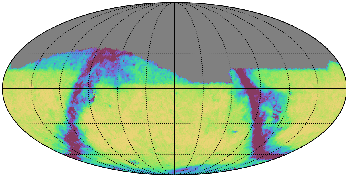
weather_cloudso4v3.4_10yrs Yr 1 r band: Exgal_CoaddM5
