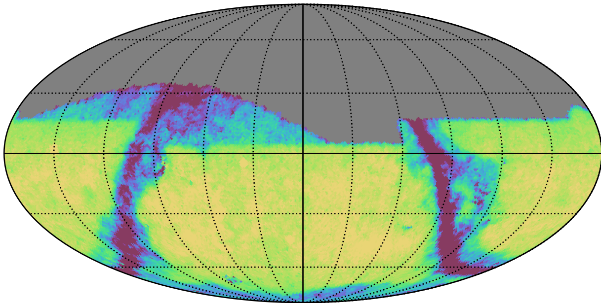
weather_cloudso4v3.4_10yrs Yr 1 i band: Exgal_CoaddM5
