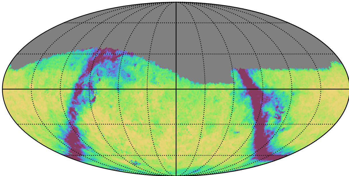
weather_cloudso4v3.4_10yrs Yr 1 g band: Exgal_CoaddM5
