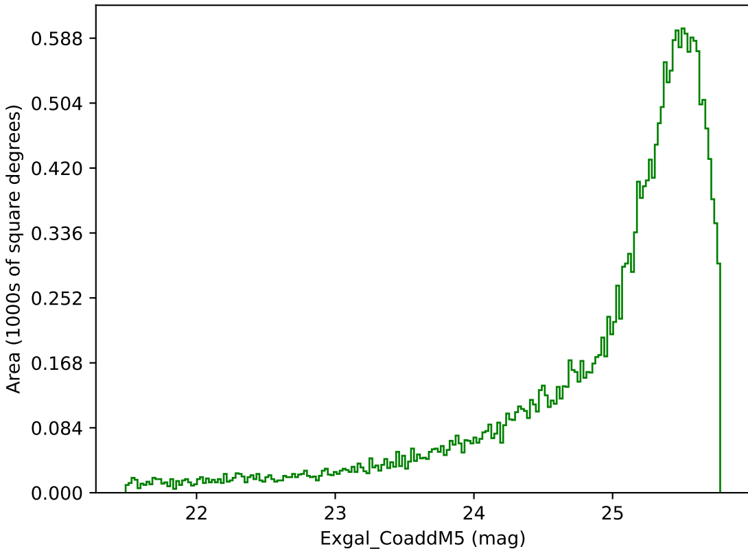
weather_cloudso4v3.4_10yrs Yr 1 g band: Exgal_CoaddM5
