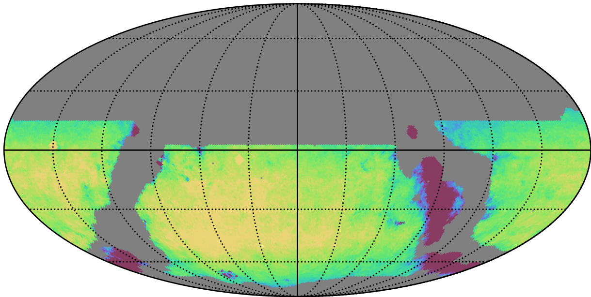
weather_cloudso4v3.4_10yrs WFD z band: Exgal_CoaddM5
