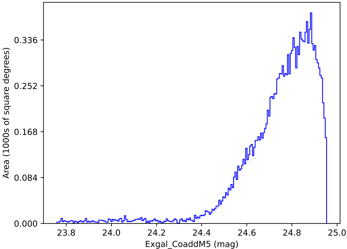
weather_cloudso4v3.4_10yrs WFD y band: Exgal_CoaddM5
