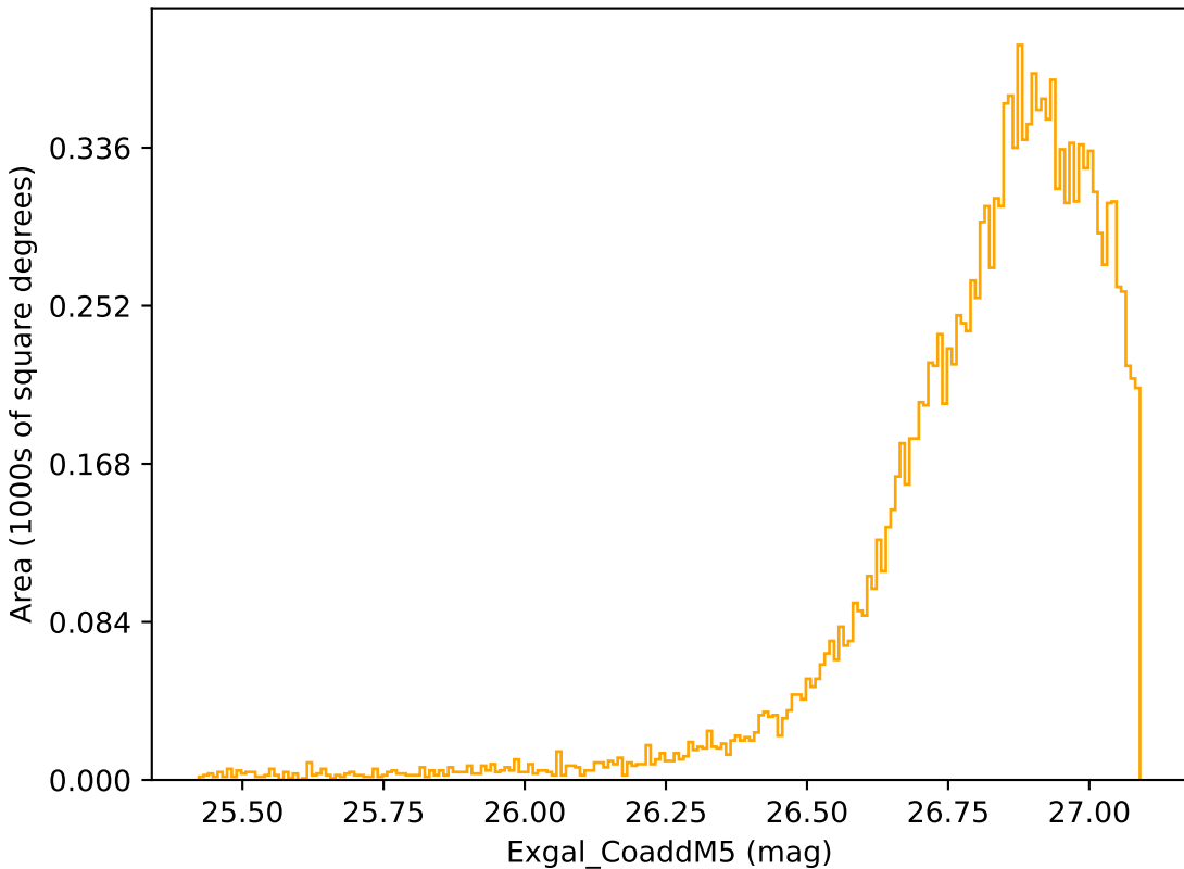
weather_cloudso4v3.4_10yrs WFD r band: Exgal_CoaddM5
