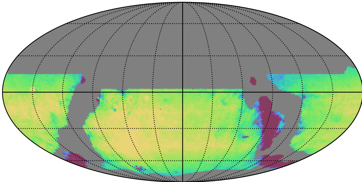
weather_cloudso4v3.4_10yrs WFD i band: Exgal_CoaddM5
