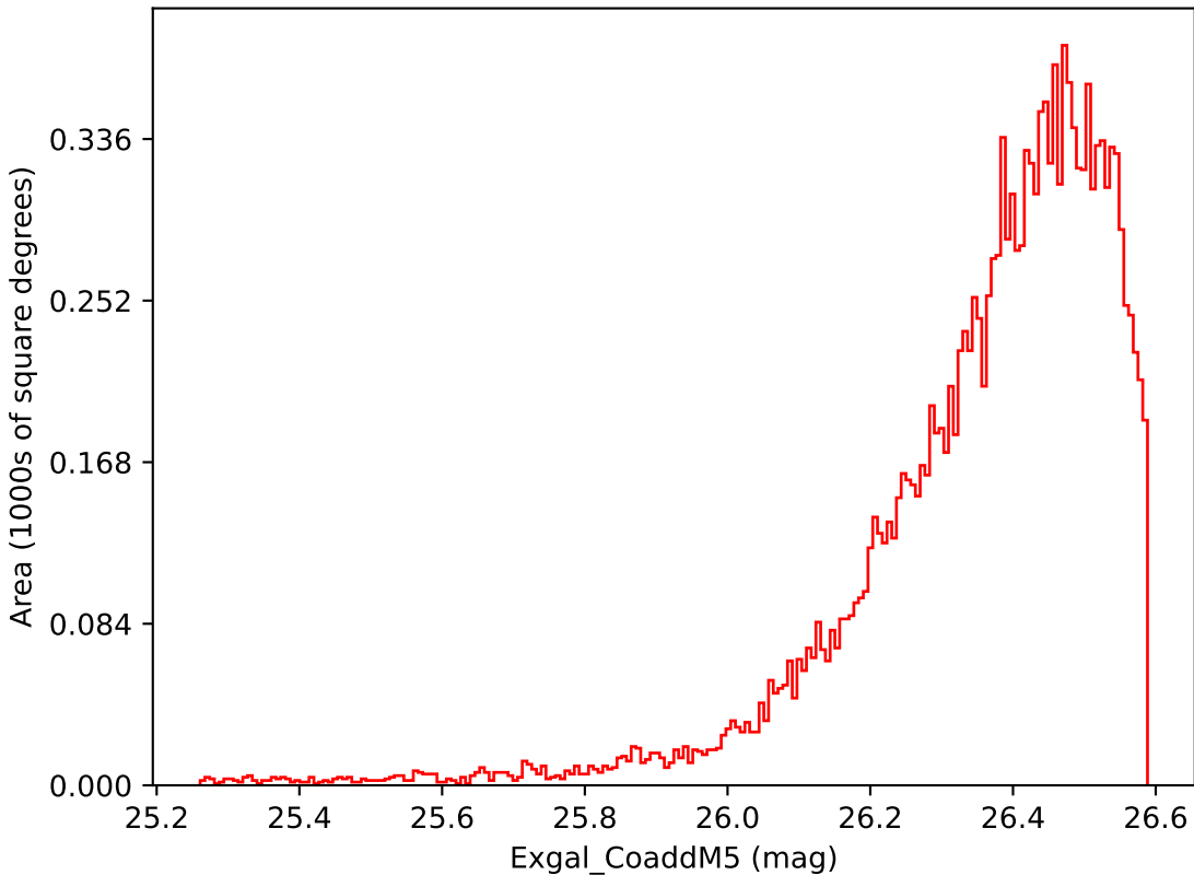
weather_cloudso4v3.4_10yrs WFD i band: Exgal_CoaddM5
