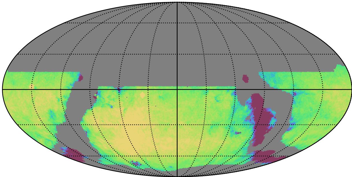
weather_cloudso4v3.4_10yrs WFD g band: Exgal_CoaddM5
