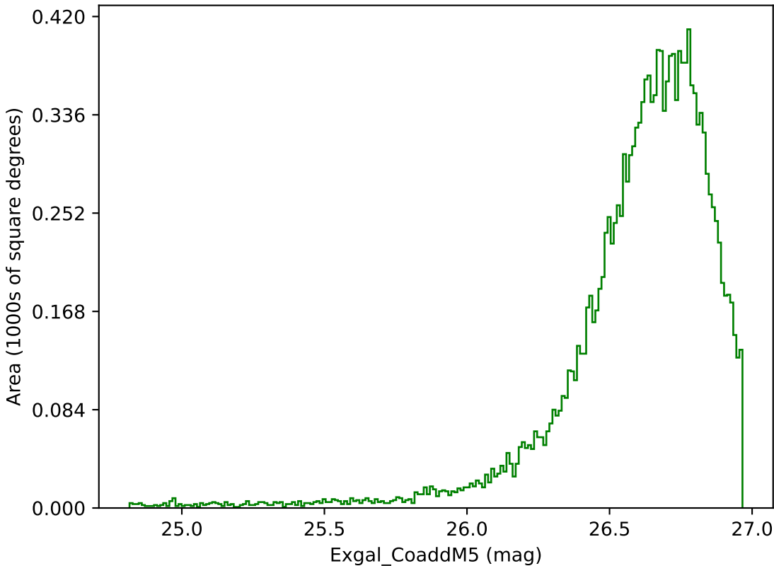
weather_cloudso4v3.4_10yrs WFD g band: Exgal_CoaddM5
