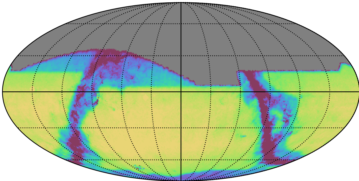
weather_cloudso4v3.4_10yrs All sky z band: Exgal_CoaddM5
