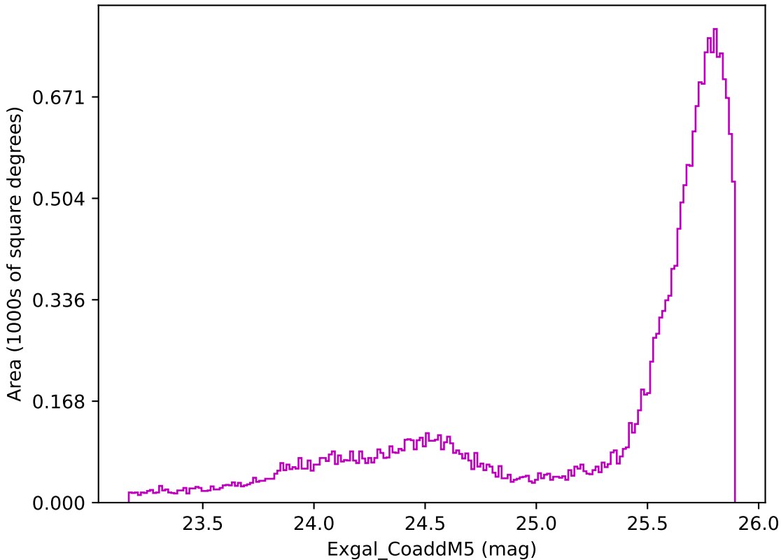
weather_cloudso4v3.4_10yrs All sky z band: Exgal_CoaddM5
