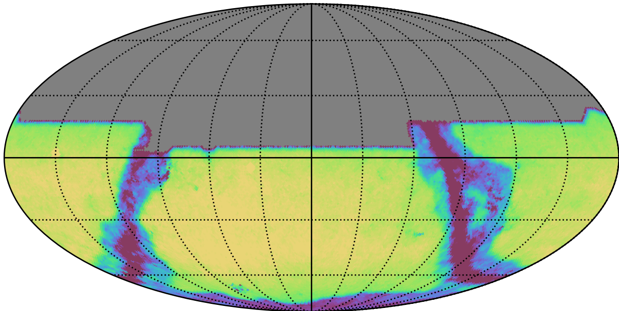
weather_cloudso4v3.4_10yrs All sky y band: Exgal_CoaddM5
