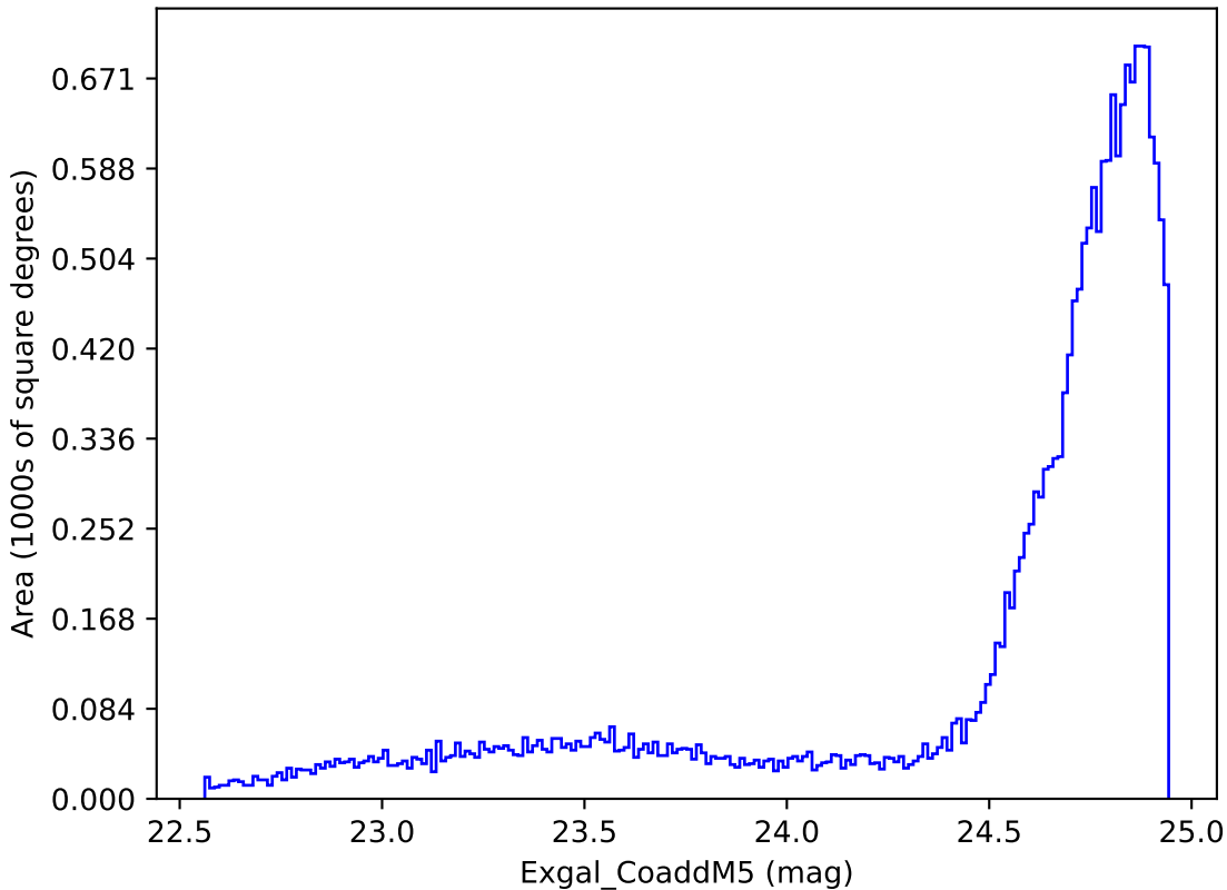
weather_cloudso4v3.4_10yrs All sky y band: Exgal_CoaddM5
