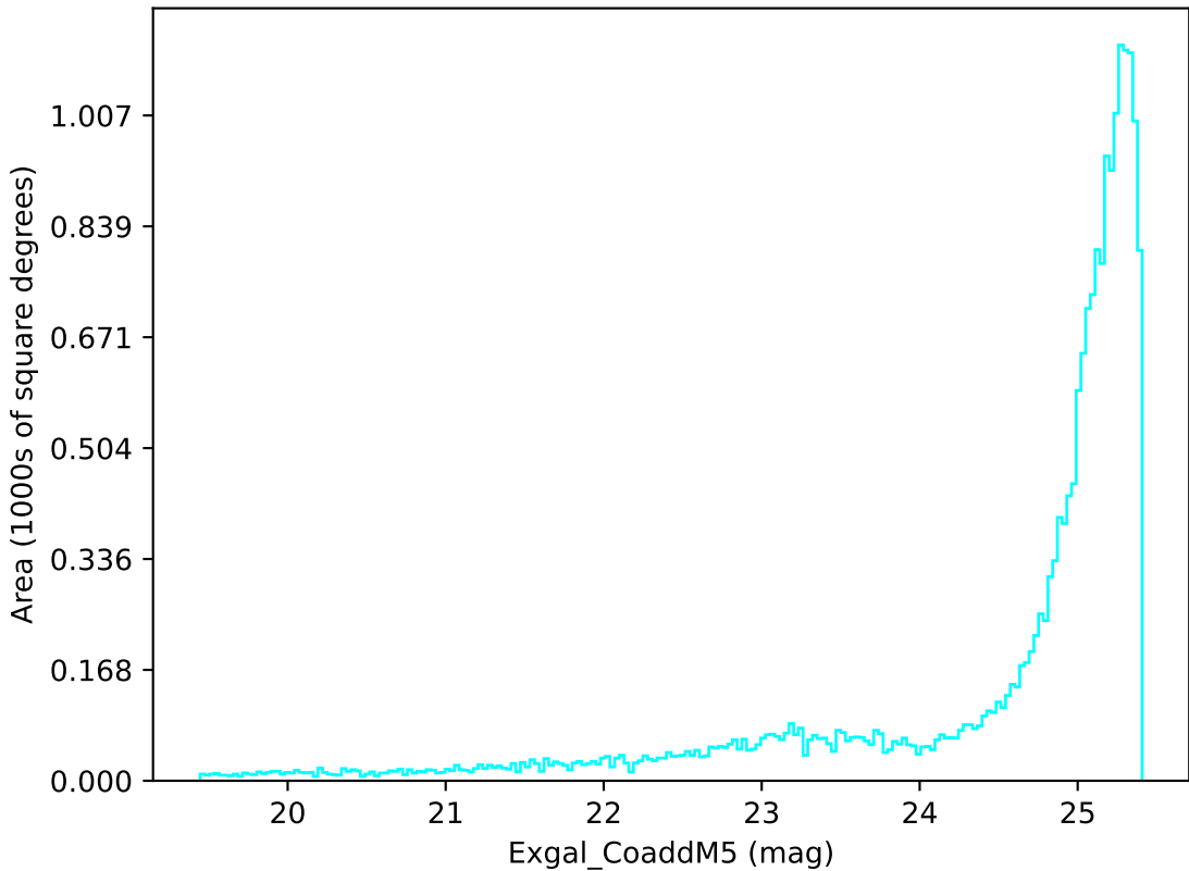
weather_cloudso4v3.4_10yrs All sky u band: Exgal_CoaddM5
