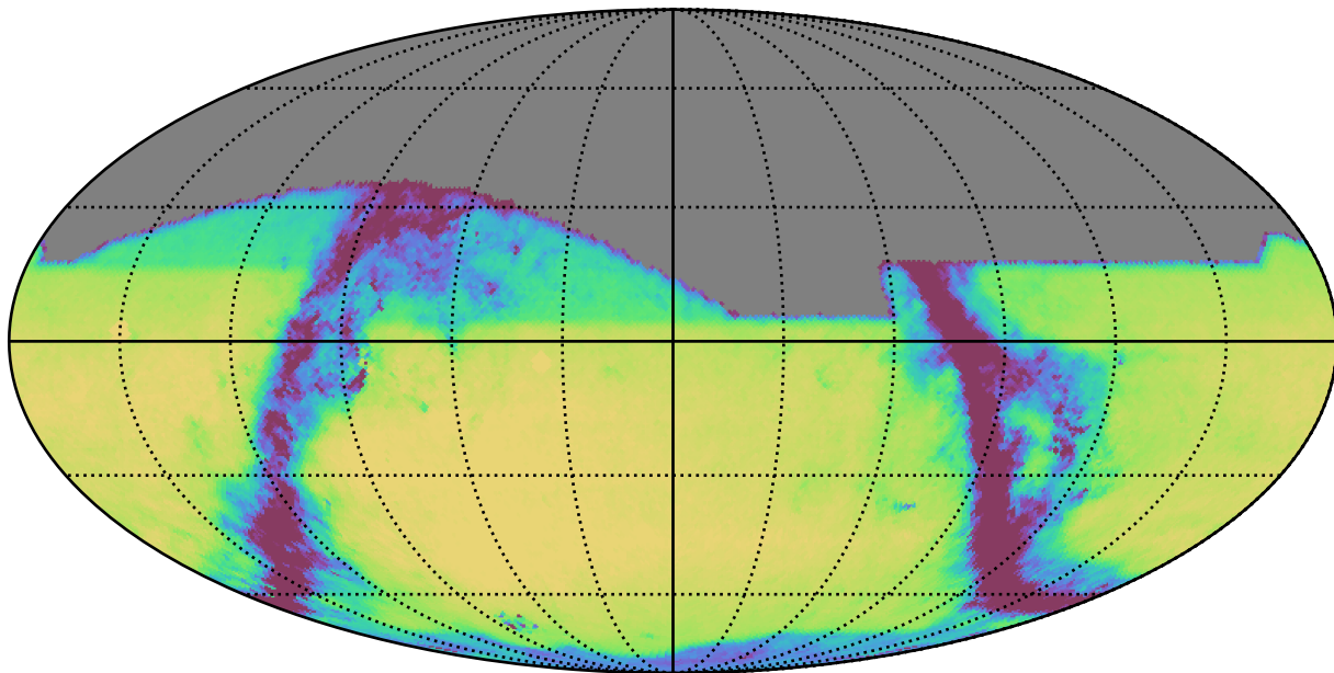
weather_cloudso4v3.4_10yrs All sky r band: Exgal_CoaddM5
