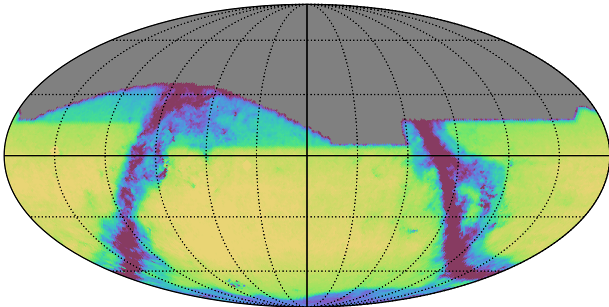
weather_cloudso4v3.4_10yrs All sky i band: Exgal_CoaddM5
