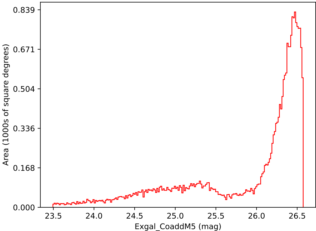
weather_cloudso4v3.4_10yrs All sky i band: Exgal_CoaddM5
