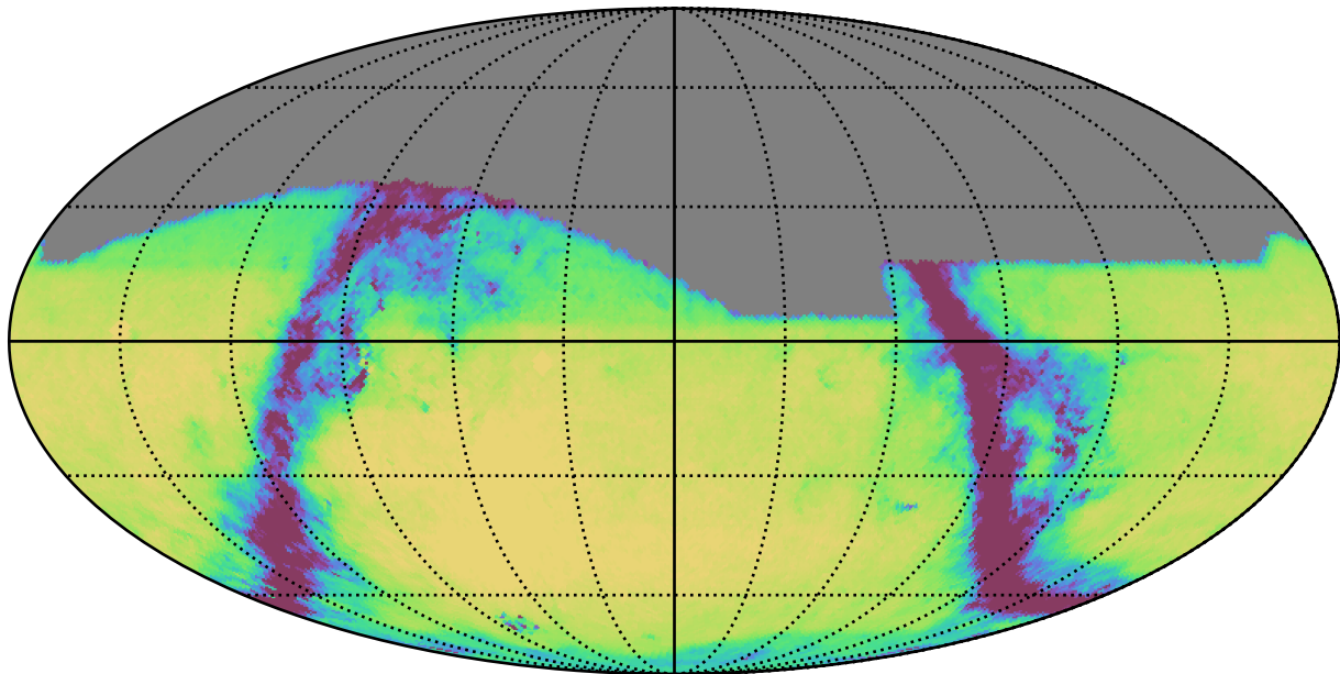
weather_cloudso4v3.4_10yrs All sky g band: Exgal_CoaddM5
