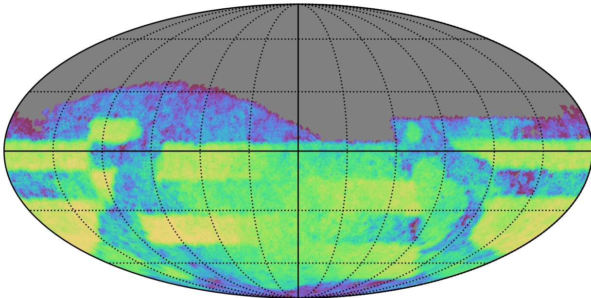
weather_cloudso4v3.4_10yrs Yr 3-4 z band: CoaddM5
