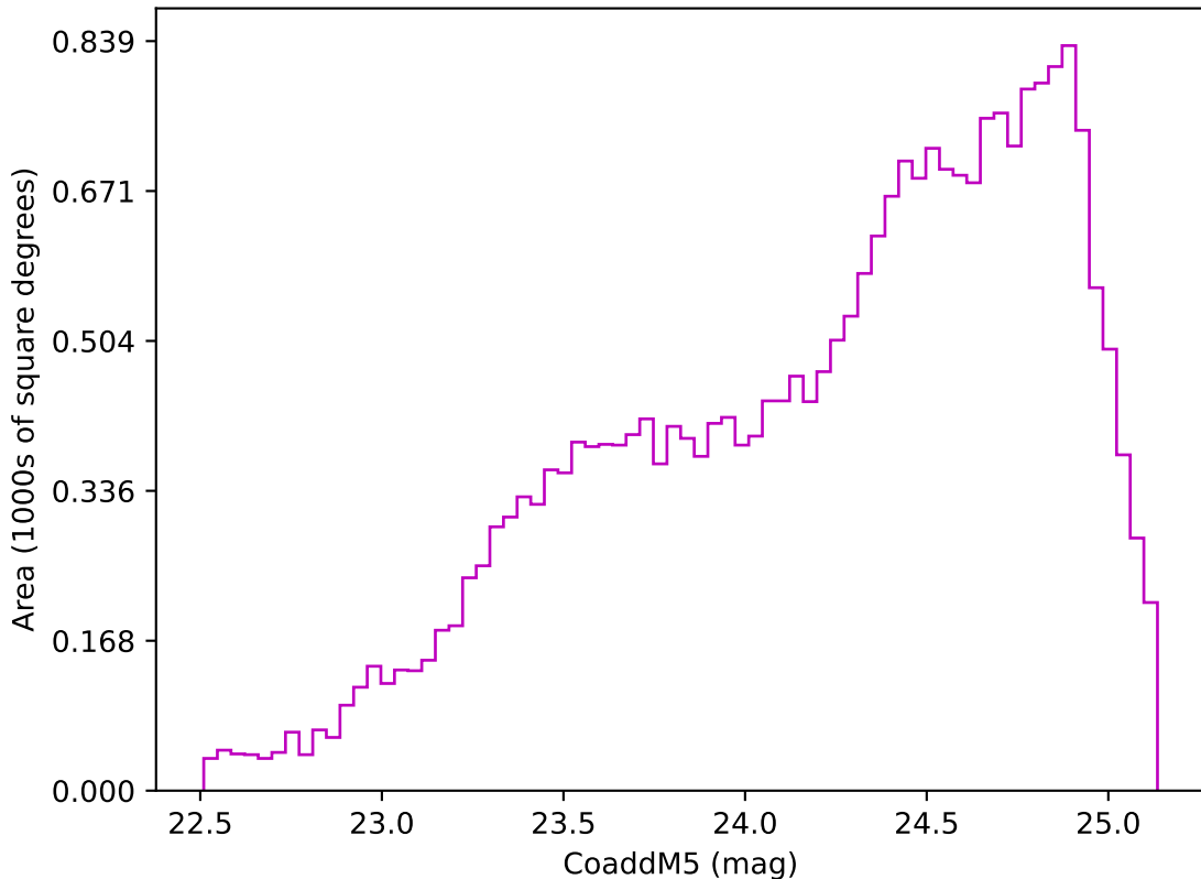
weather_cloudso4v3.4_10yrs Yr 3-4 z band: CoaddM5
