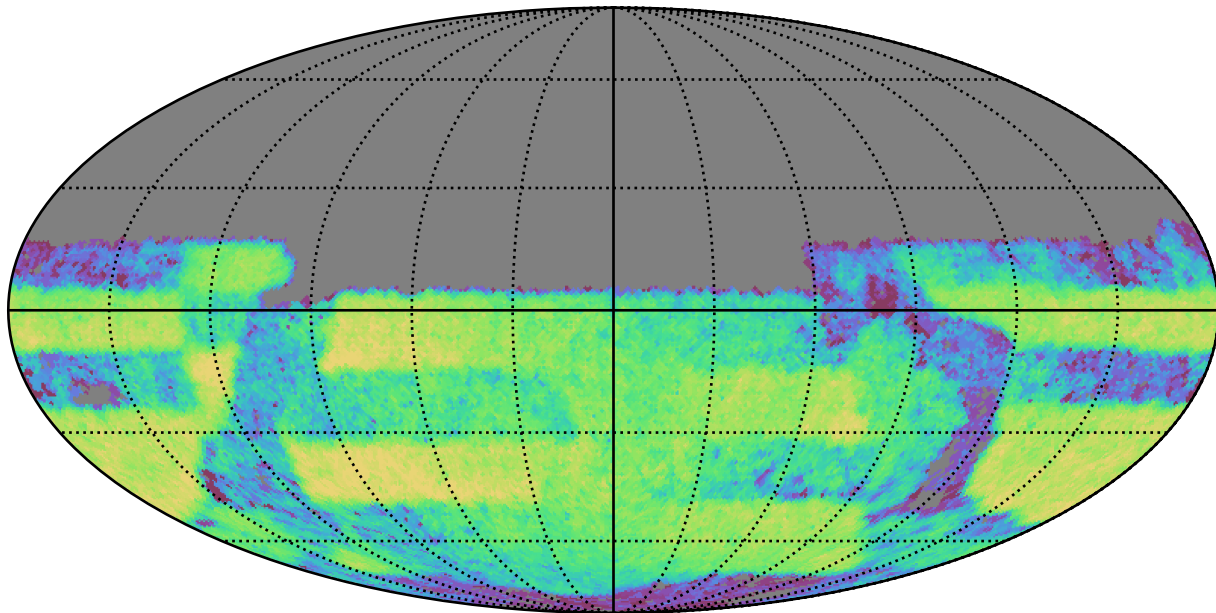
weather_cloudso4v3.4_10yrs Yr 3-4 y band: CoaddM5
