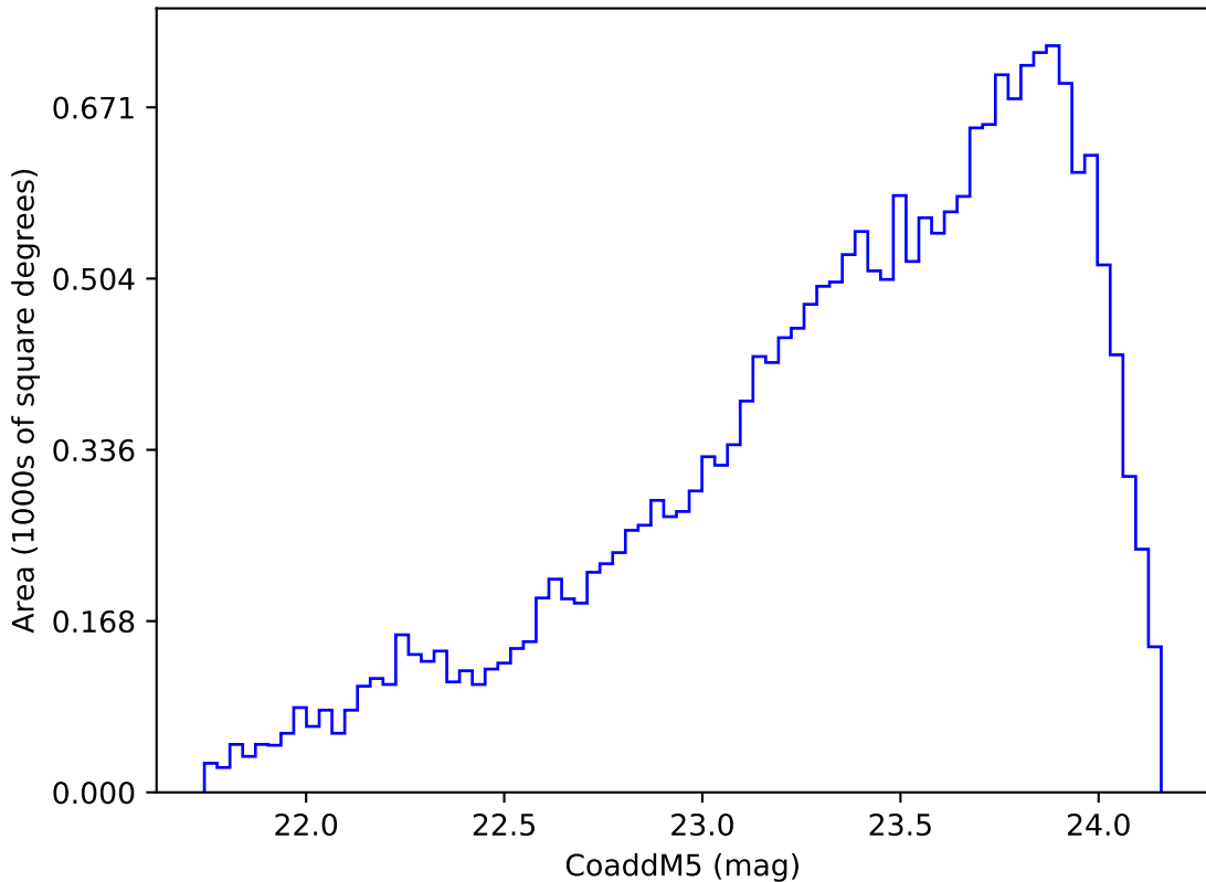
weather_cloudso4v3.4_10yrs Yr 3-4 y band: CoaddM5
