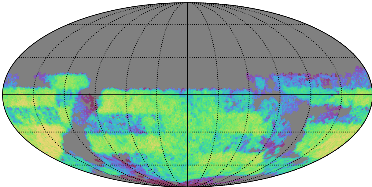
weather_cloudso4v3.4_10yrs Yr 3-4 u band: CoaddM5
