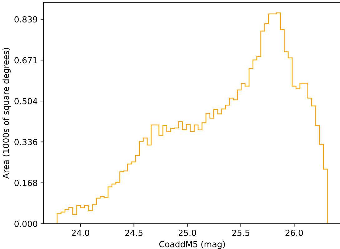
weather_cloudso4v3.4_10yrs Yr 3-4 r band: CoaddM5
