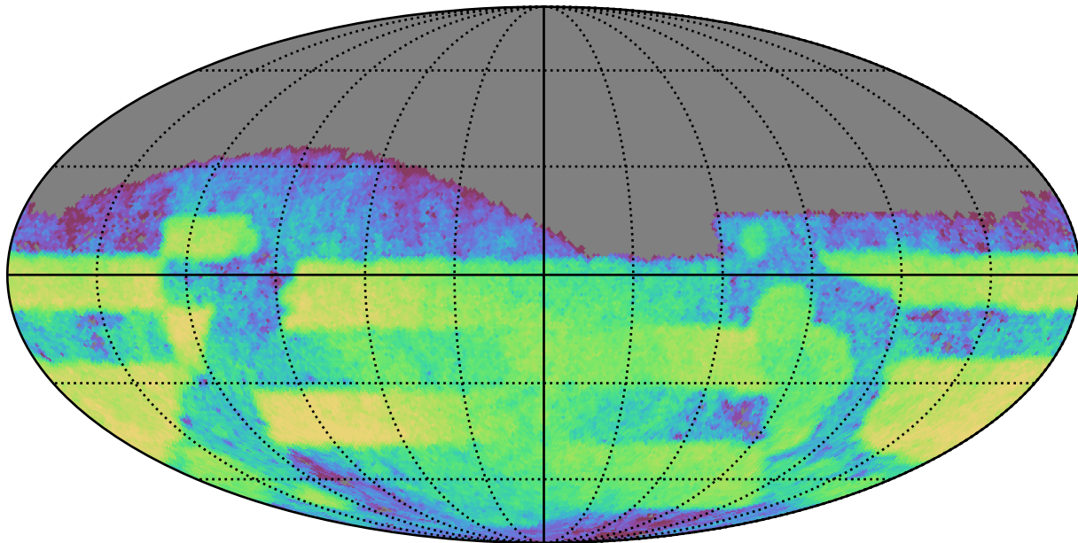
weather_cloudso4v3.4_10yrs Yr 3-4 i band: CoaddM5
